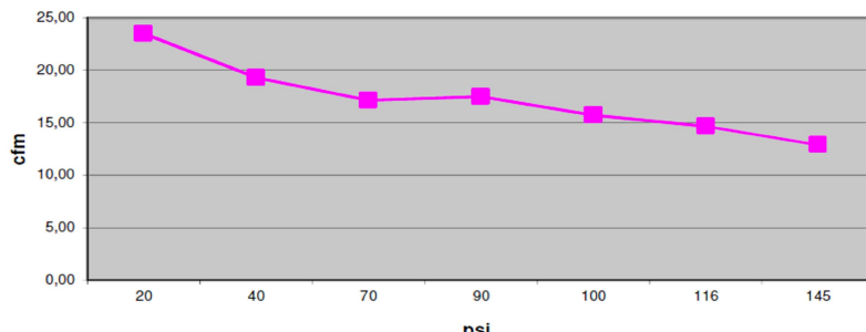
Air Flow Chart
